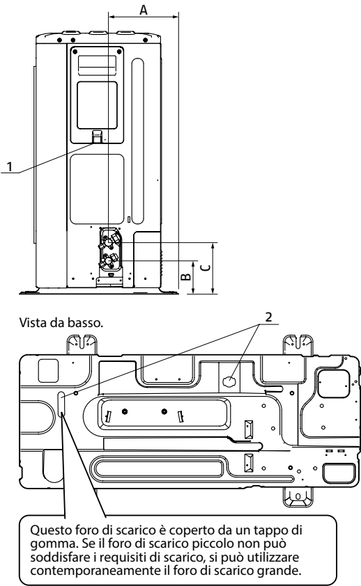
HP EXTERNAL UNIT 008÷016 - 012T÷016T
