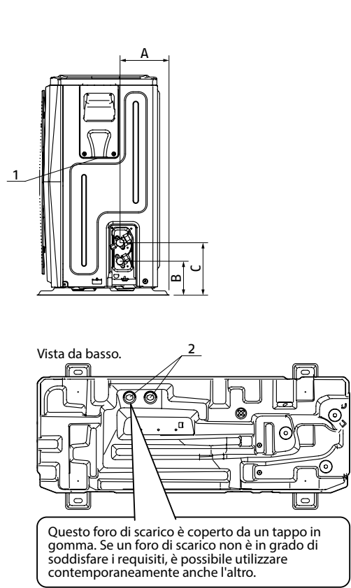
HP EXTERNAL UNIT 004-006
